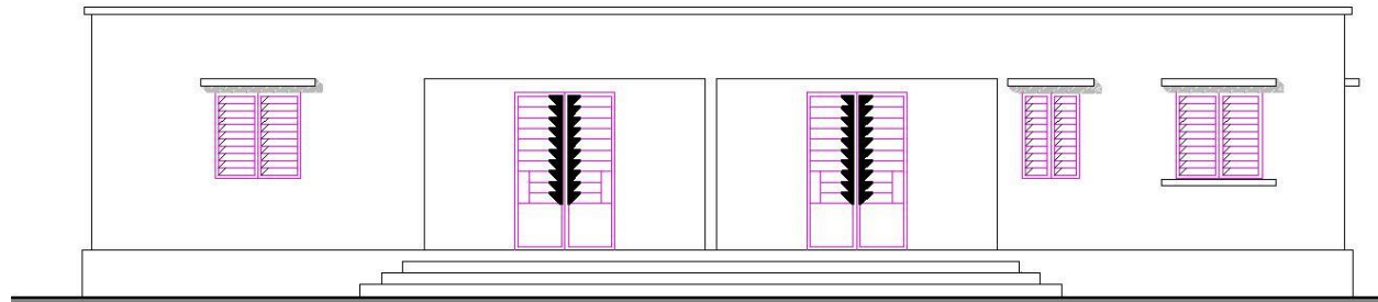
FAÇADE PRINCIPALE
