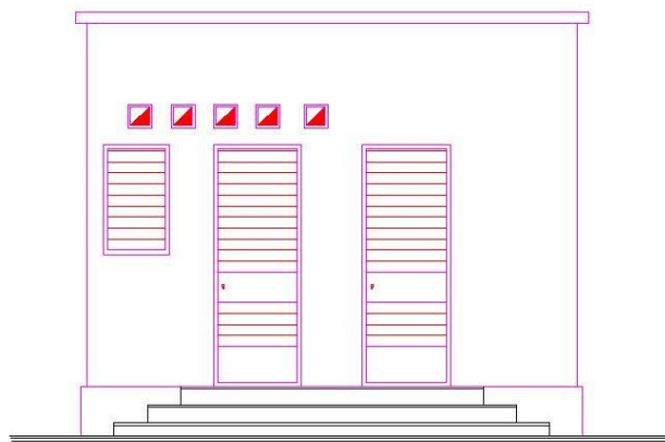
FAÇADE
